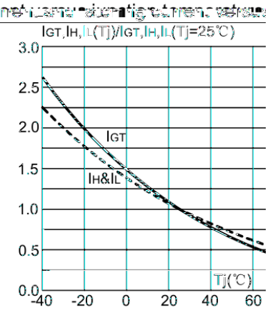
FIG.4: Relative variations of gate trigger current, holding current and latching current vs. temperature
