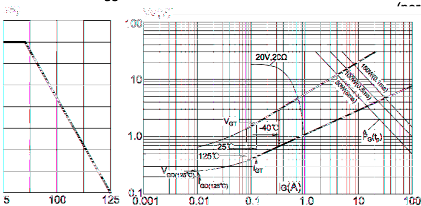
FIG.5 Gate trigger characteristics
