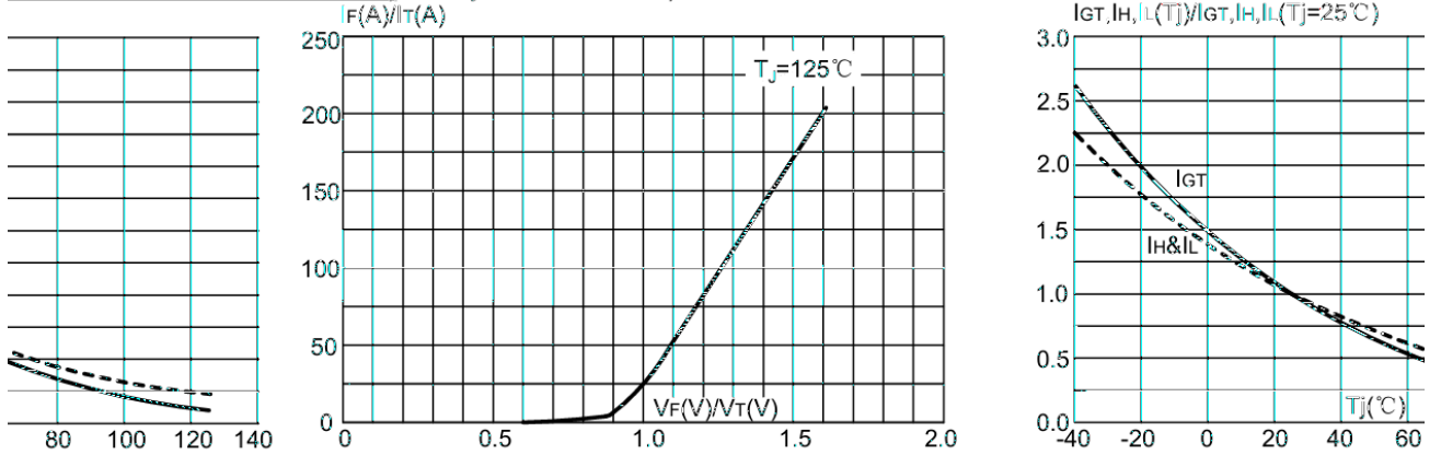
FIG.5: Gate trigger characteristics
