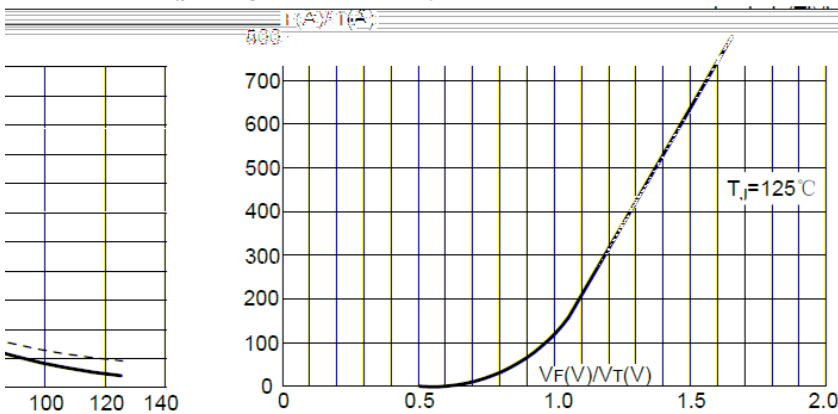
FIG.3: Forward characteristics (per thyristor or diode)
