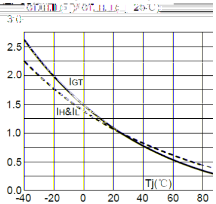
FIG.4: Relative variations of gate trigger current, holding current and latching current versus junction temperature
