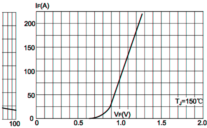
FIG.1: Forward characteristics (at T_J = 150^\circ\text{C} )
