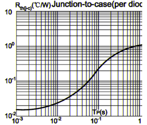
FIG.4: Maximum transient thermal in
