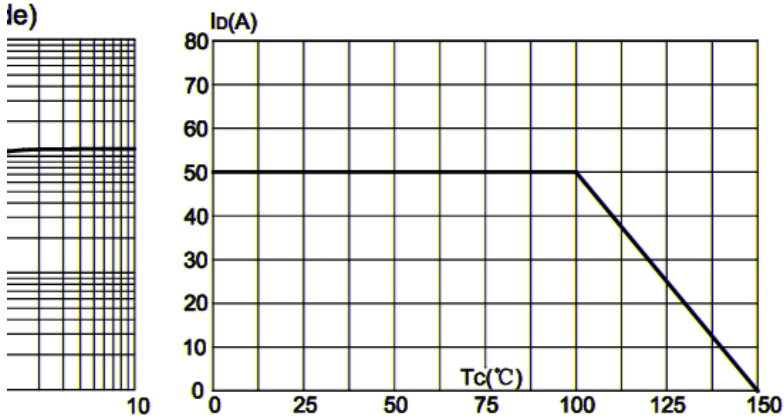
FIG.3: Forward current vs. case temperature
