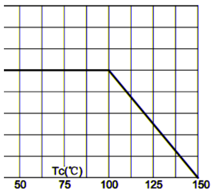
Forward current vs. case temperature
