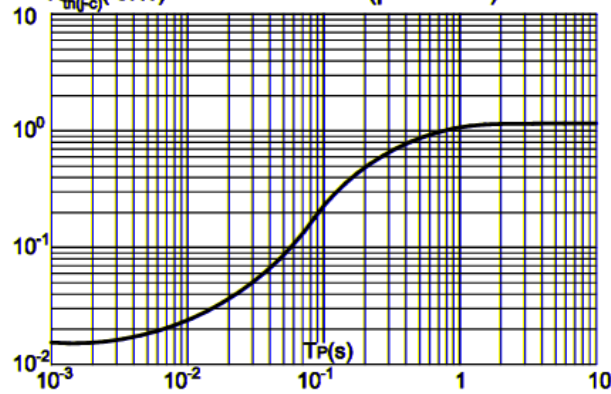
FIG.4: Maximum transient thermal impedance R_{th(j-c)} ( ^\circ\text{C/W} ) Junction-to-case(per diode)
