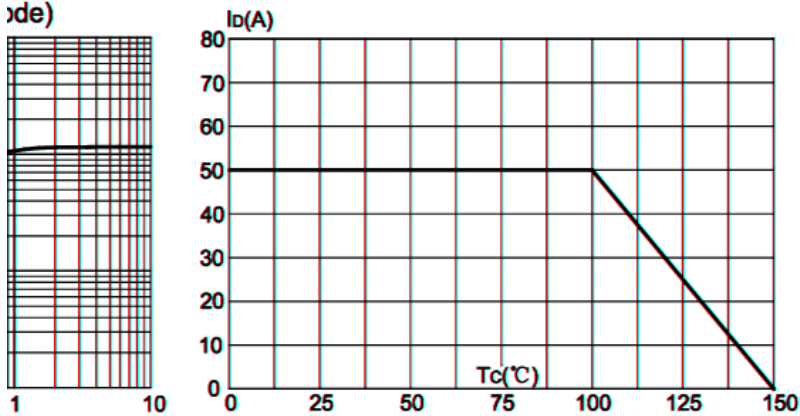
FIG.3: Forward current vs. case temperature
