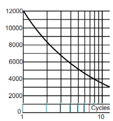
FIG.2: Peak on-state surge current
