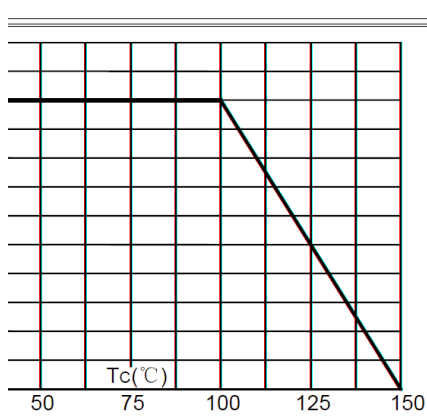
FIG.3: Forward current vs. case temperature
