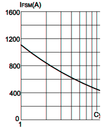
FIG.2: Peak on-state surge current
