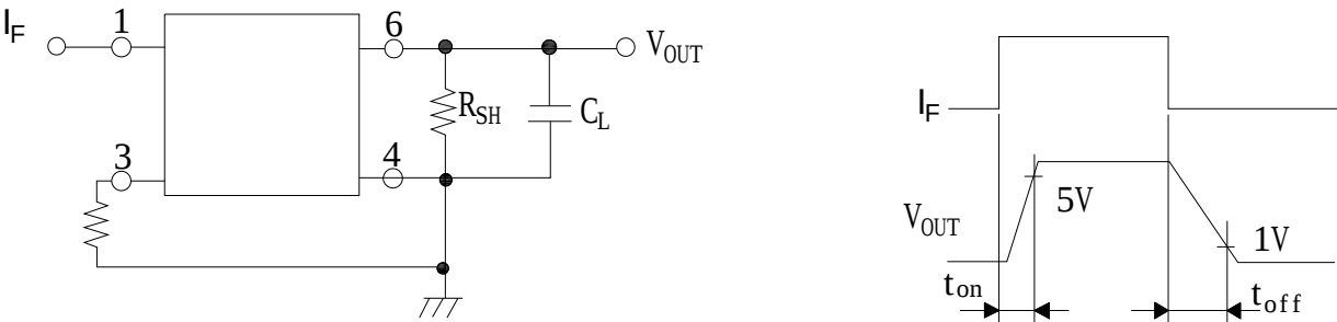
FIG.7: Response Time Test Circuit, Waveform
