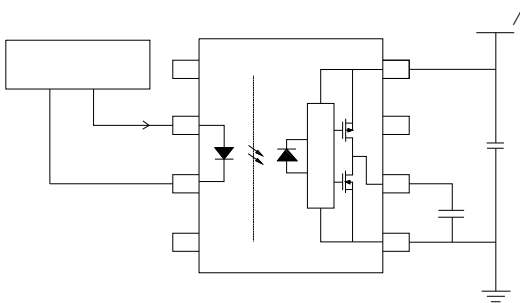
Fig.9: Test Circuits for TPHL, TPLH, tr, tf
