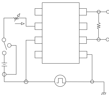
Fig.10: CMTI Test Circuit and Waveform
